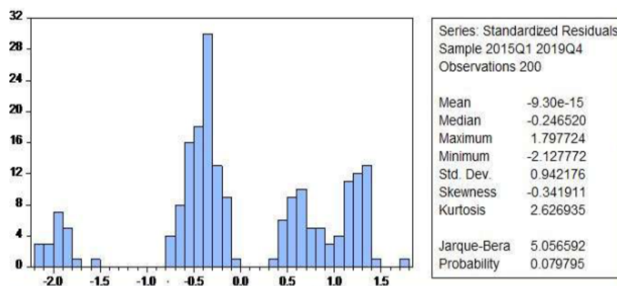
Figure 2 Normality Test with the Test of Jarque-Bera
